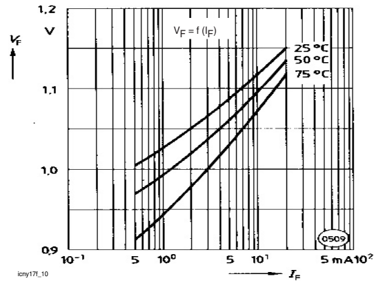
Figure 10. Forward Voltage
